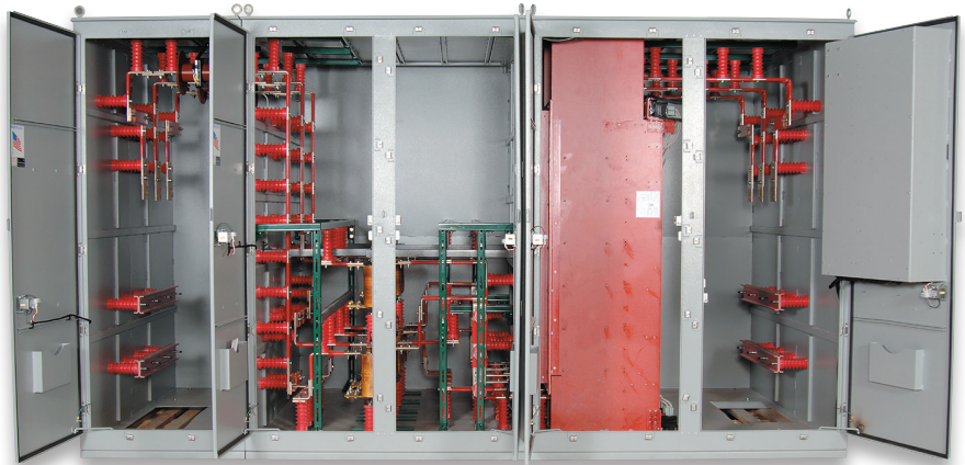
20 MW, 13.8 kV
