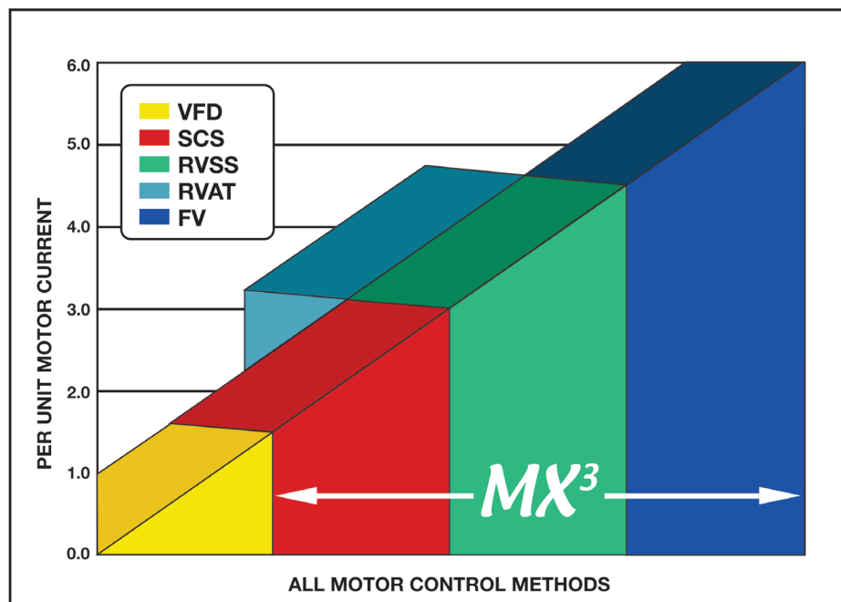
FIGURE 2. Starting current comparison.
