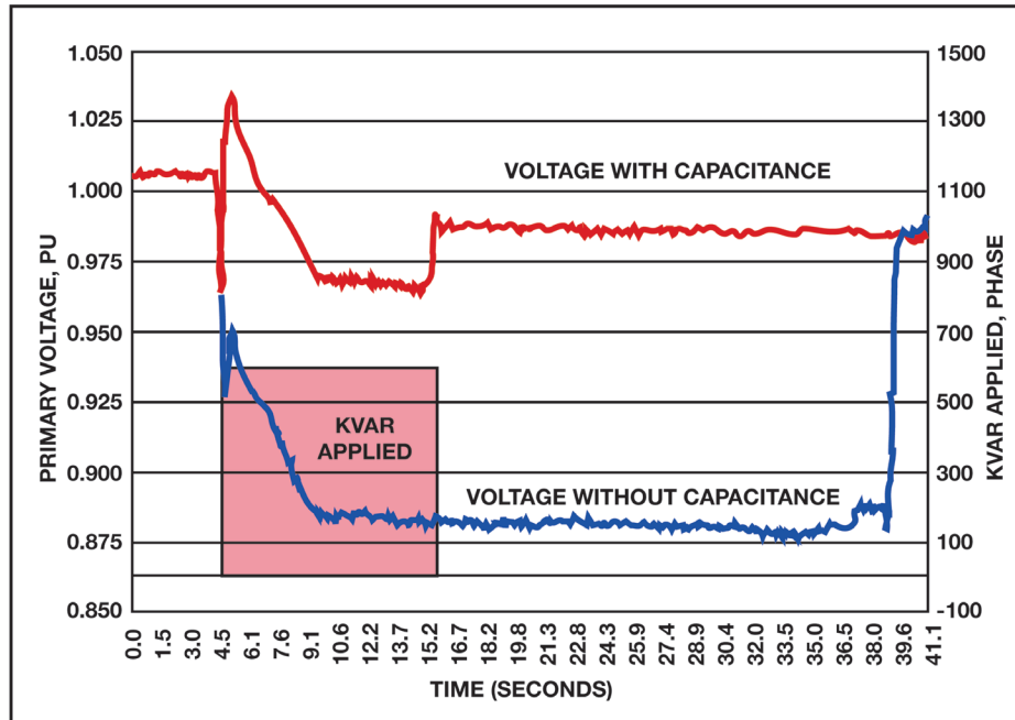
FIGURE 1. Motor start comparison with and without capacitance.
